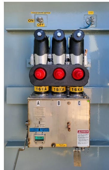
HV RADIAL FEED
